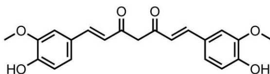
Figure 1. Chemical Structure of Curcumin (diferuloylmethane)
