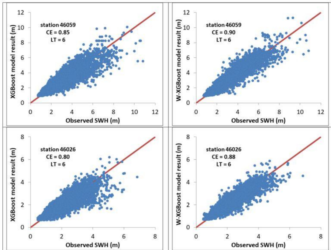
Fig. 5 Stand-alone XGBoost and W-XGBoost model results for 6 hour leadtime and stations 46059 and 46026, respectively.
